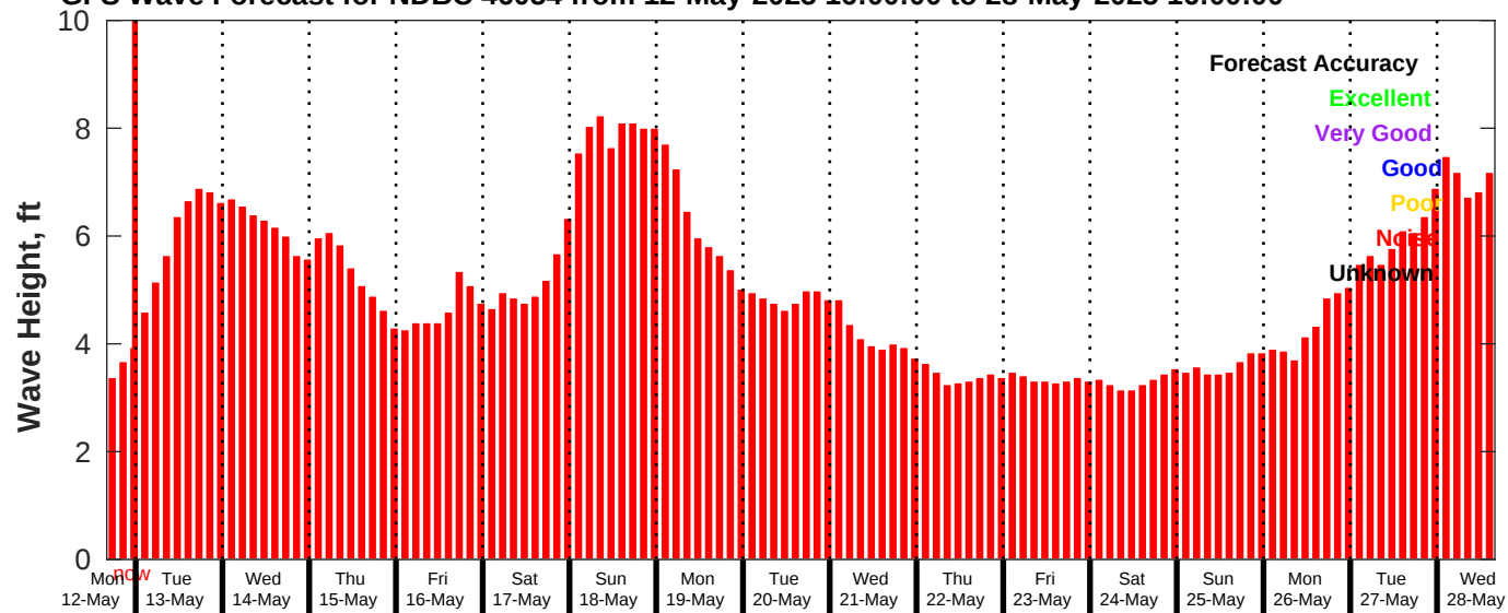
GFS Wave Forecast for NDBC 46054 from 12-May-2025 16:00:00 to 28-May-2025 16:00:00
