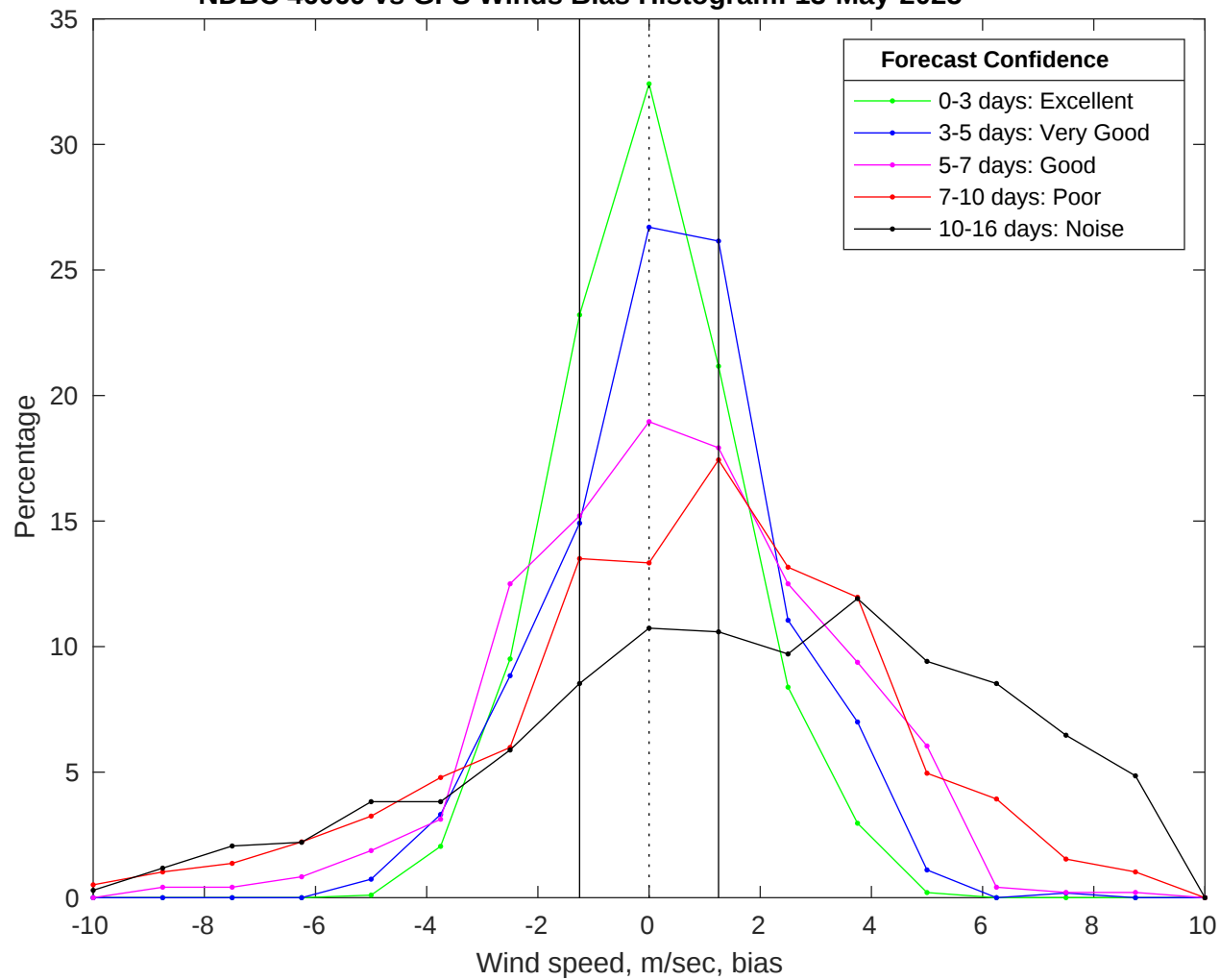
NDBC 46069 vs GFS Winds Bias Histogram: 13-May-2025
