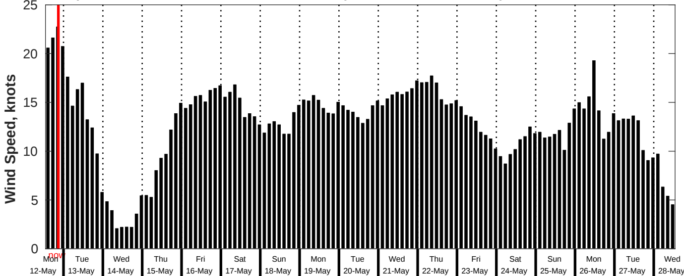
GFS Wind Speed Forecast for NDBC 51209 from 12-May-2025 13:00:00 to 28-May-2025 13:00:00
