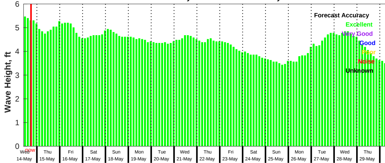
GFS Wave Forecast for NDBC 52211 from 13-May-2025 10:00:00 to 29-May-2025 10:00:00
