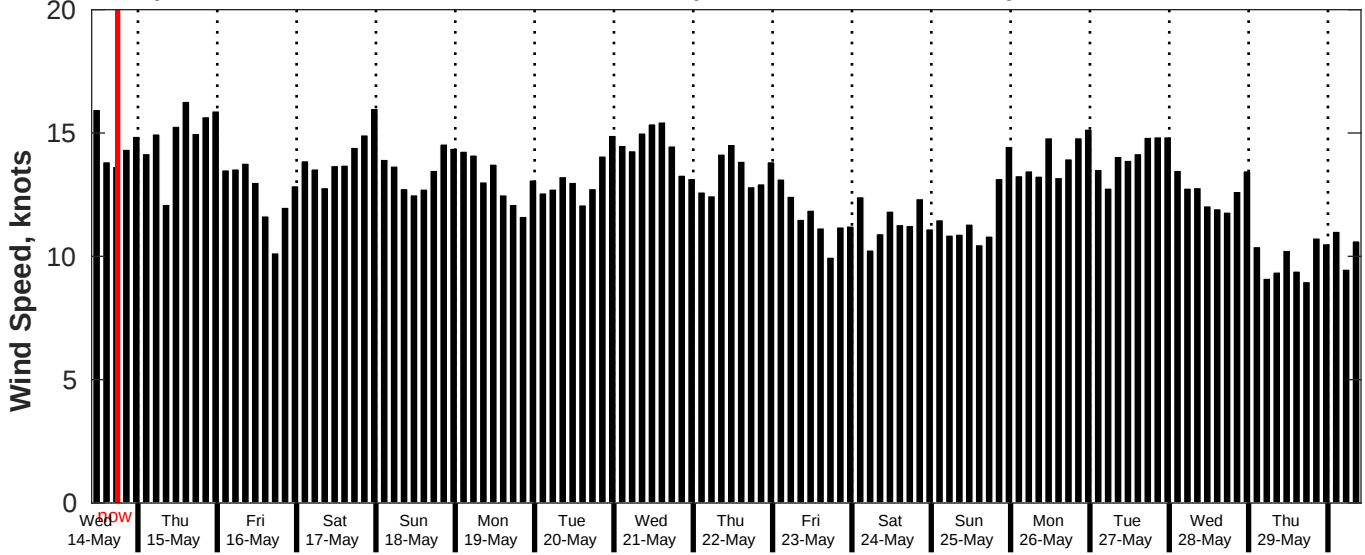
GFS Wind Speed Forecast for NDBC 52211 from 13-May-2025 10:00:00 to 29-May-2025 10:00:00
