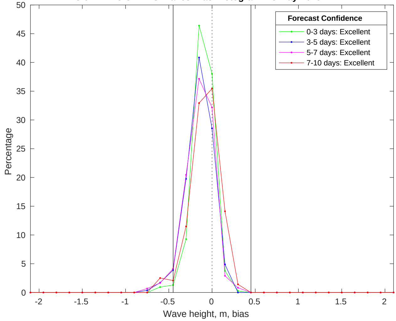
NDBC 52212 vs CMEMS Waves Bias Histogram: 13-May-2025
