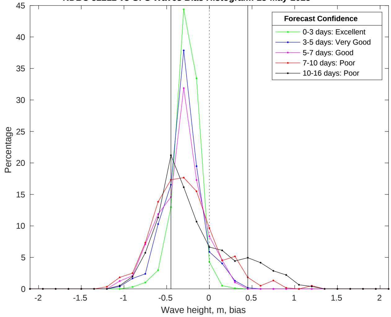
NDBC 52212 vs GFS Waves Bias Histogram: 13-May-2025
