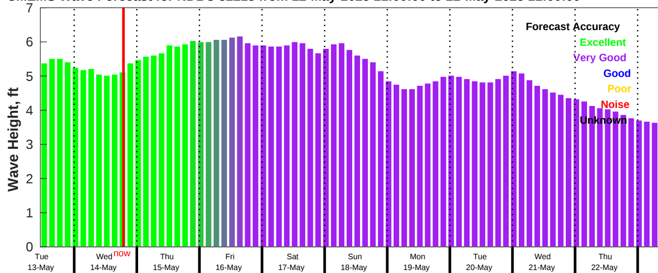
CEEMS Wave Forecast for NDBC 52213 from 12-May-2025 11:00:00 to 22-May-2025 11:00:00
