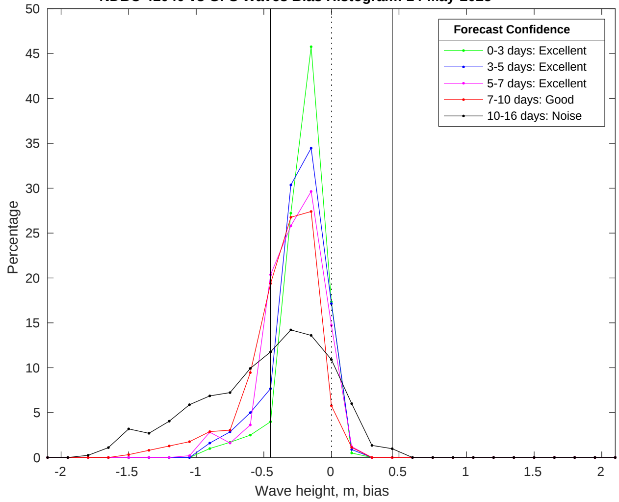
NDBC 41040 vs GFS Waves Bias Histogram: 14-May-2025
