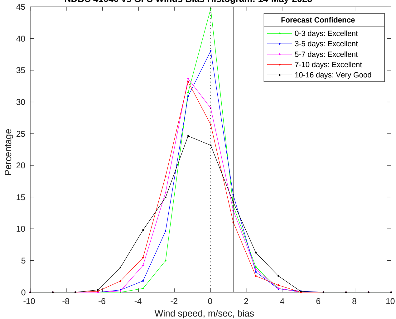
NDBC 41040 vs GFS Winds Bias Histogram: 14-May-2025
