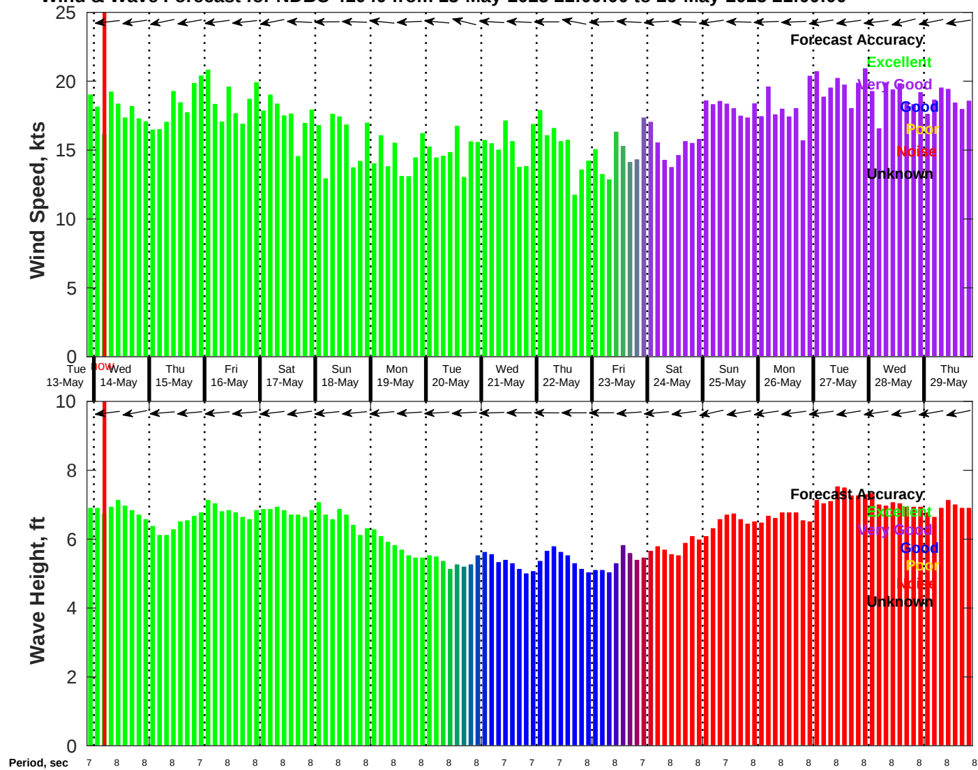
Wind & Wave Forecast for NDBC 41040 from 13-May-2025 21:00:00 to 29-May-2025 21:00:00
