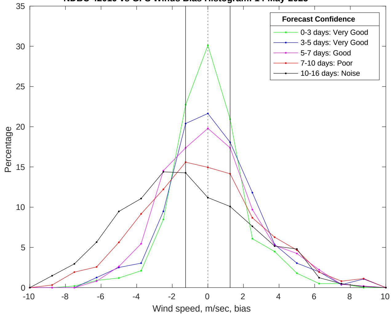
NDBC 42019 vs GFS Winds Bias Histogram: 14-May-2025
