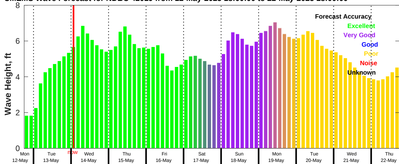
CMEMS Wave Forecast for NDBC 42019 from 12-May-2025 18:00:00 to 22-May-2025 18:00:00
