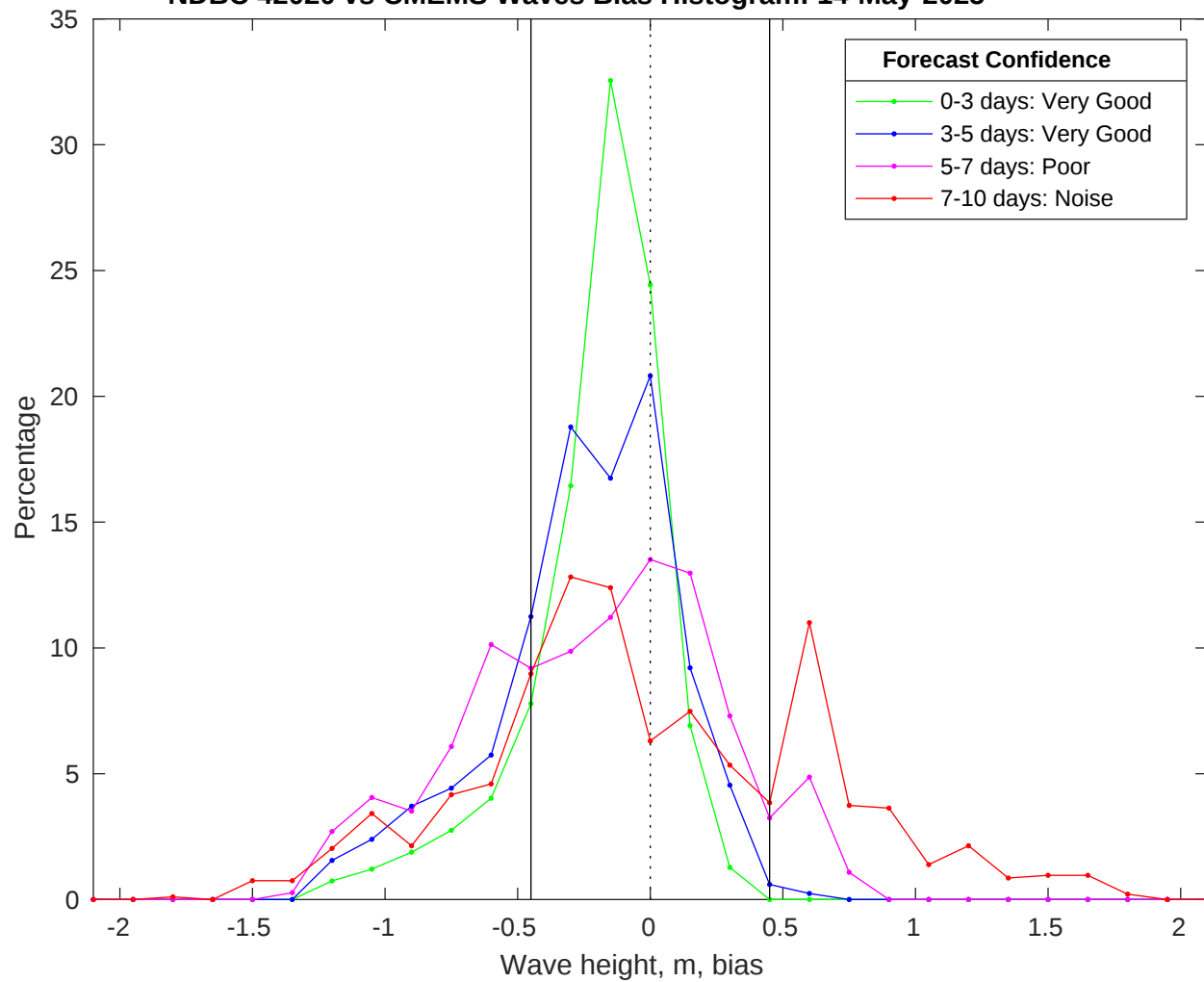
NDBC 42020 vs CMEMS Waves Bias Histogram: 14-May-2025
