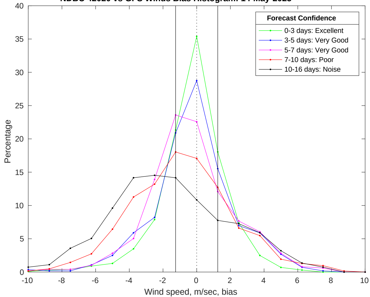
NDBC 42020 vs GFS Winds Bias Histogram: 14-May-2025
