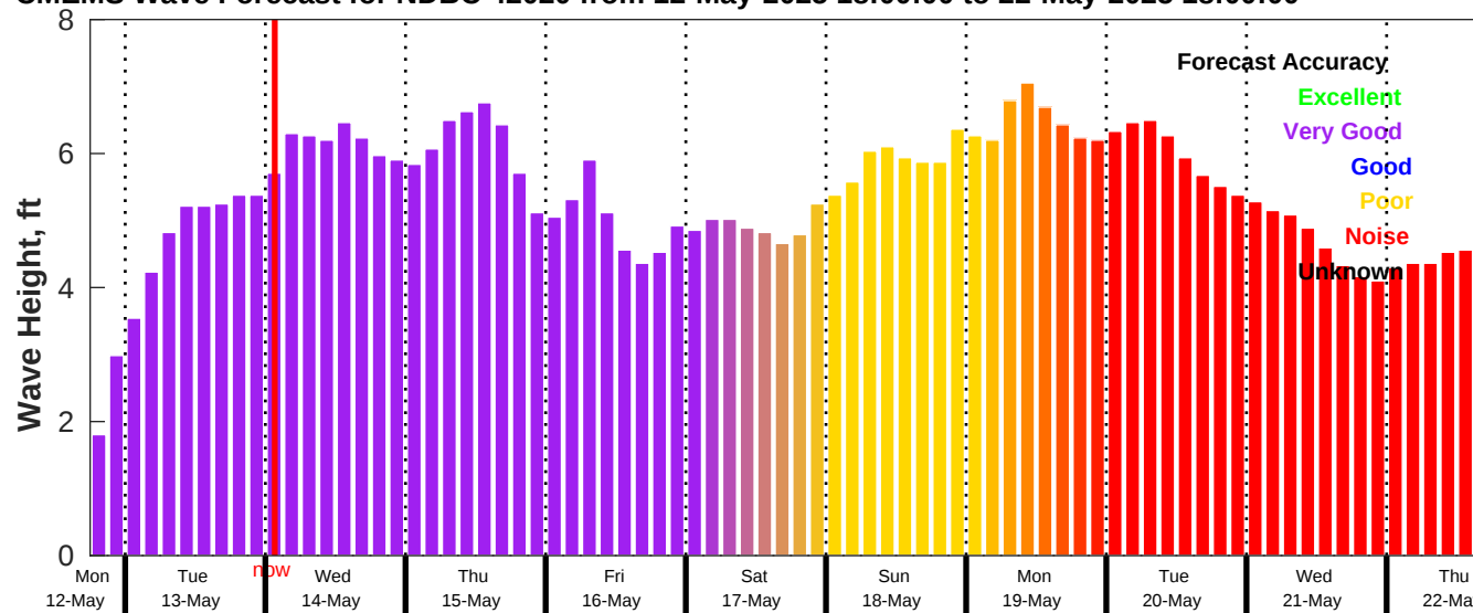
CMEMS Wave Forecast for NDBC 42020 from 12-May-2025 18:00:00 to 22-May-2025 18:00:00
