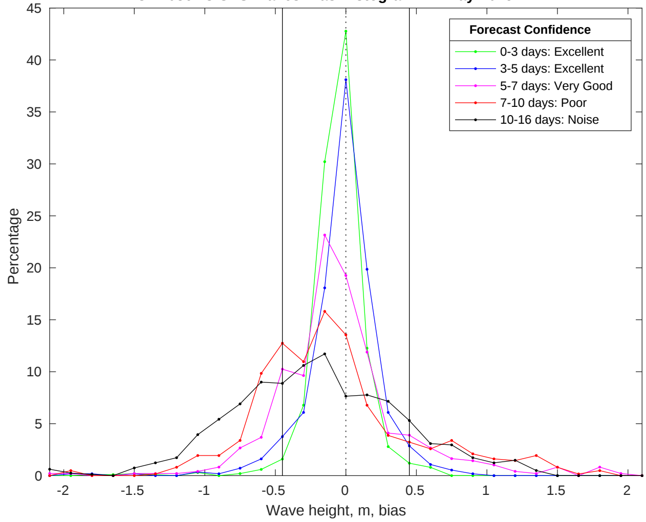
NDBC 42036 vs GFS Waves Bias Histogram: 14-May-2025
