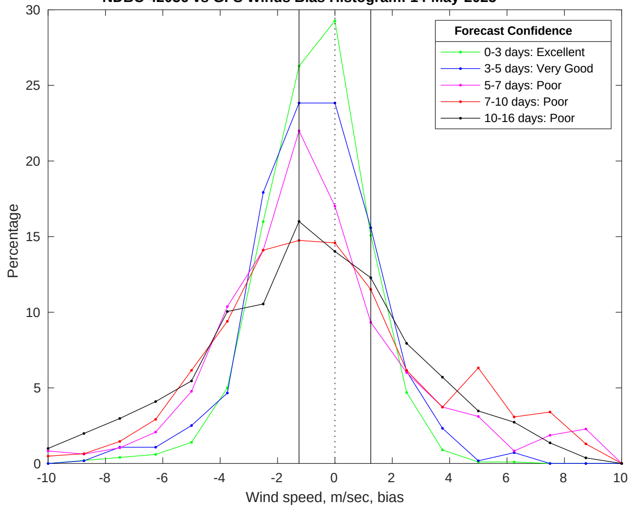
NDBC 42036 vs GFS Winds Bias Histogram: 14-May-2025
