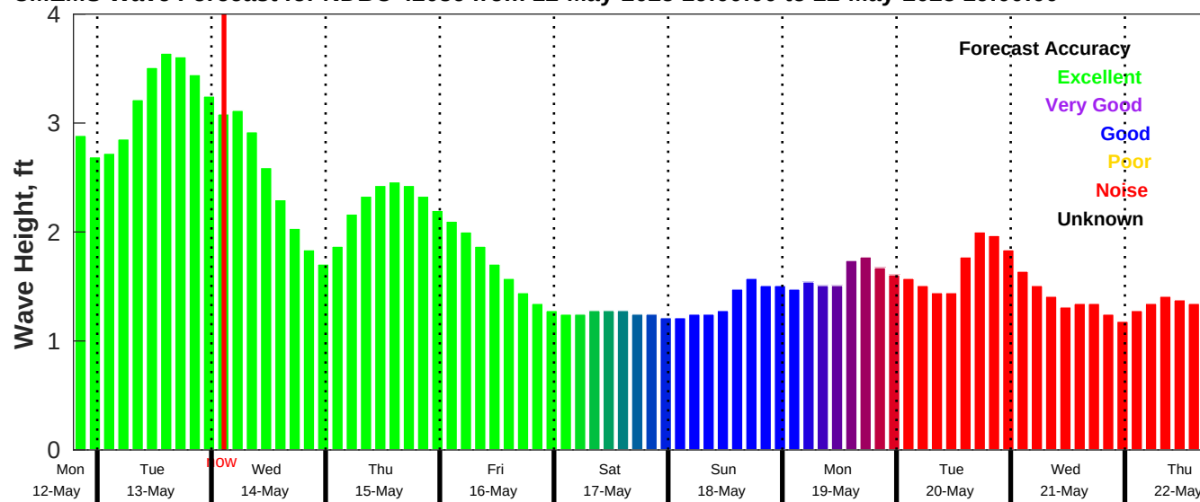
CMEMS Wave Forecast for NDBC 42036 from 12-May-2025 19:00:00 to 22-May-2025 19:00:00
