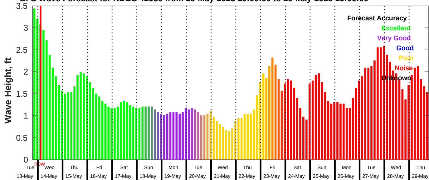
GFS Wave Forecast for NDBC 42036 from 13-May-2025 19:00:00 to 29-May-2025 19:00:00
