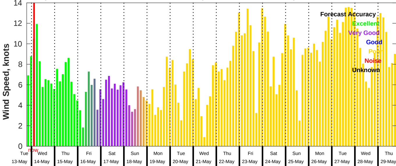
GFS Wind Speed Forecast for NDBC 42036 from 13-May-2025 19:00:00 to 29-May-2025 19:00:00
