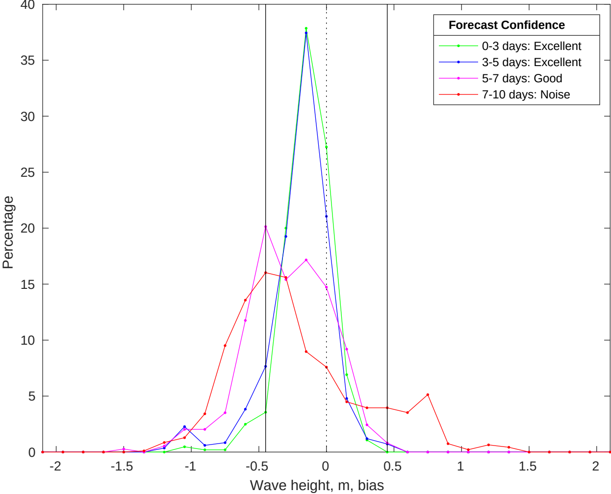
NDBC 42040 vs CMEMS Waves Bias Histogram: 14-May-2025
