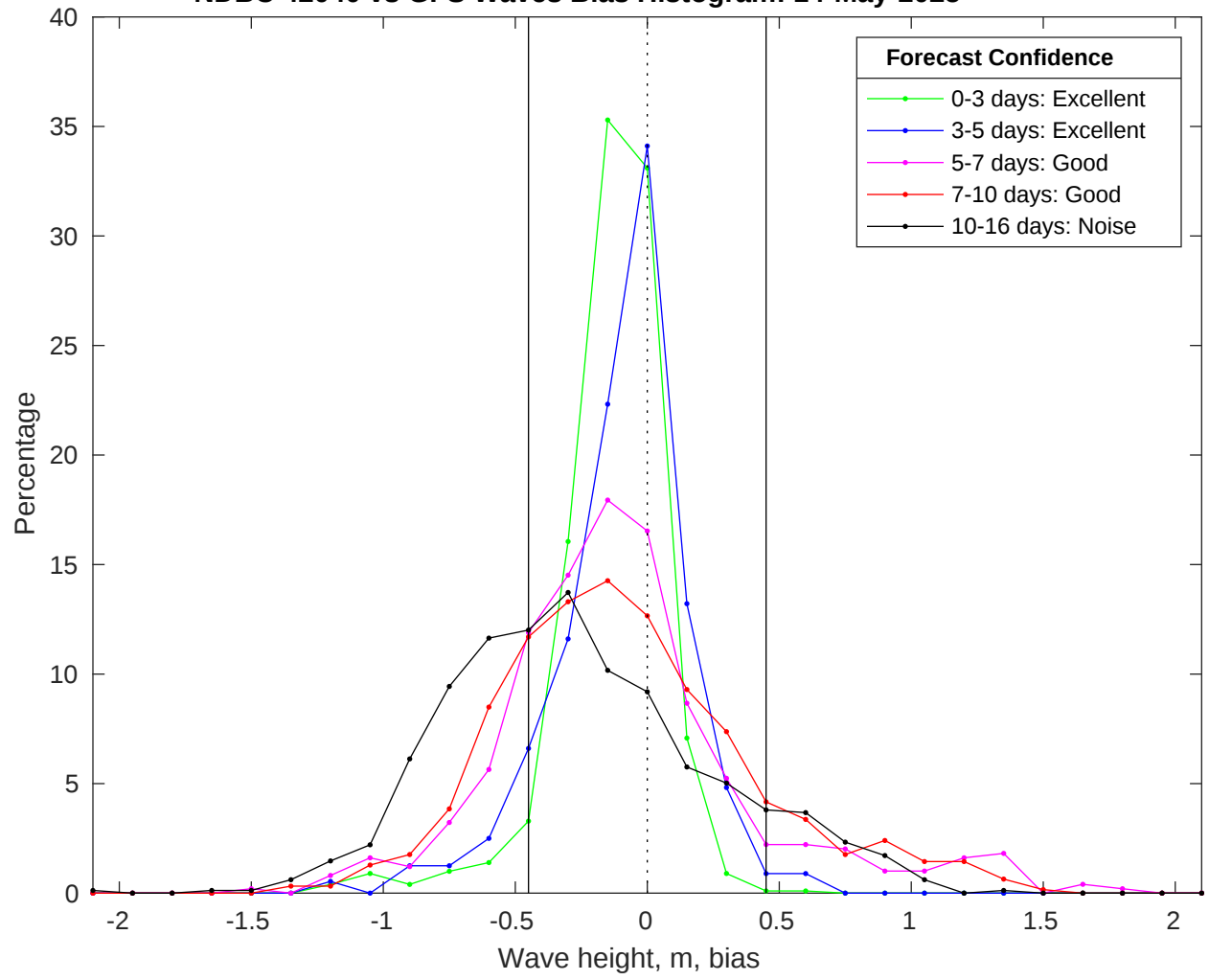
NDBC 42040 vs GFS Waves Bias Histogram: 14-May-2025
