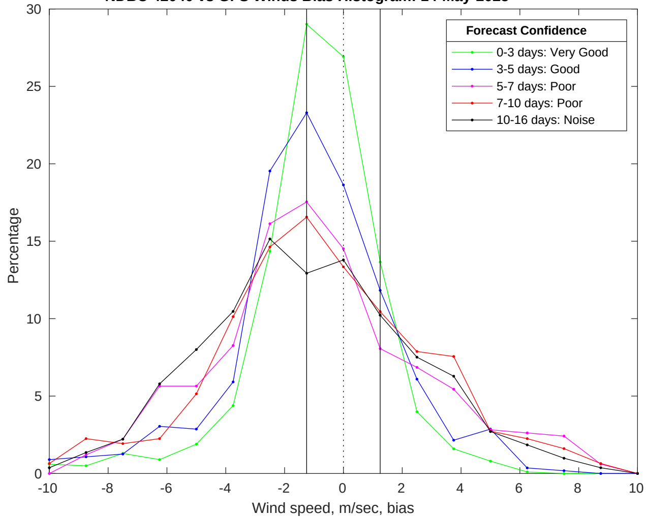
NDBC 42040 vs GFS Winds Bias Histogram: 14-May-2025
