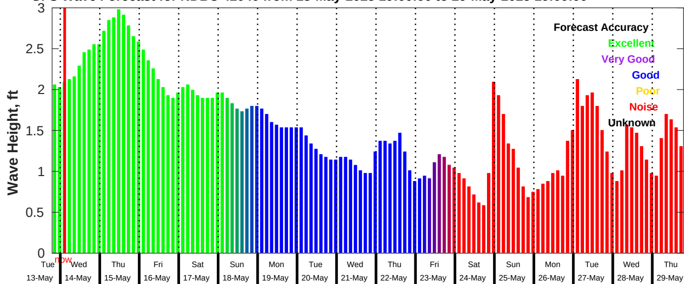
GFS Wave Forecast for NDBC 42040 from 13-May-2025 19:00:00 to 29-May-2025 19:00:00
