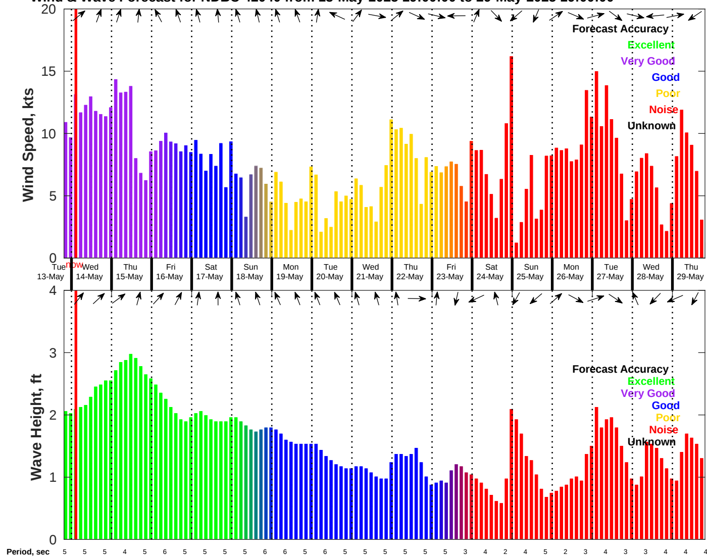
Wind & Wave Forecast for NDBC 42040 from 13-May-2025 19:00:00 to 29-May-2025 19:00:00
