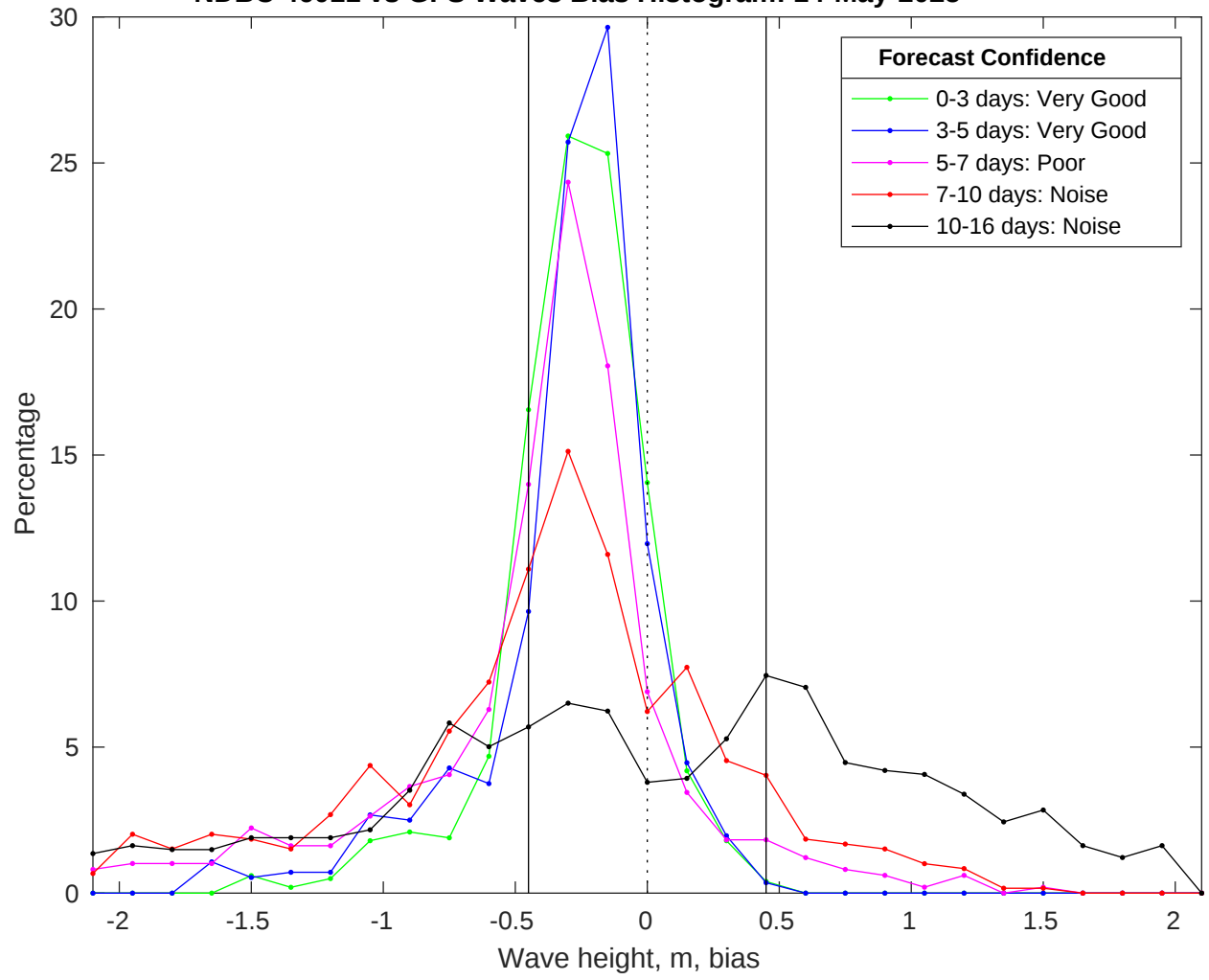
NDBC 46011 vs GFS Waves Bias Histogram: 14-May-2025
