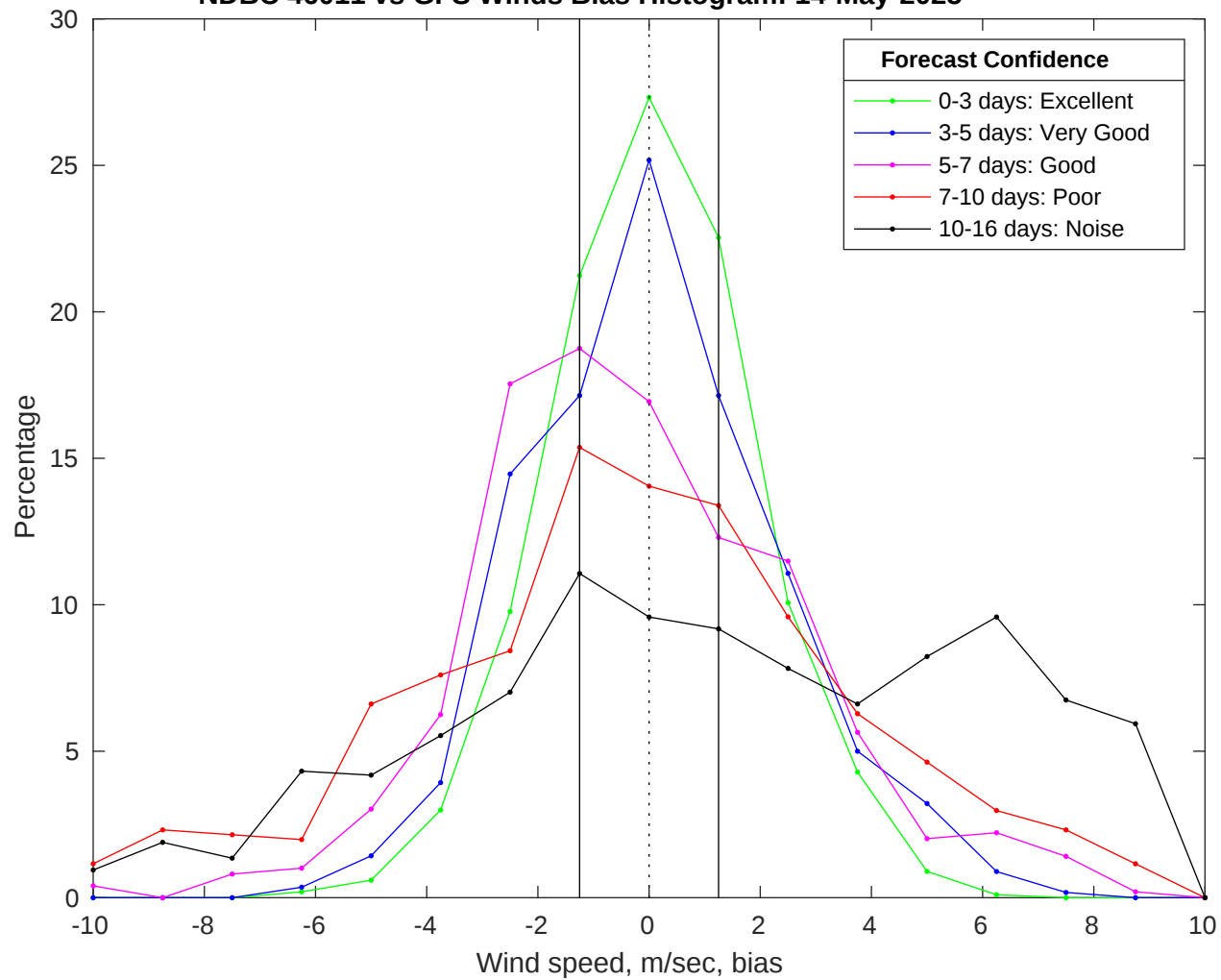
NDBC 46011 vs GFS Winds Bias Histogram: 14-May-2025
