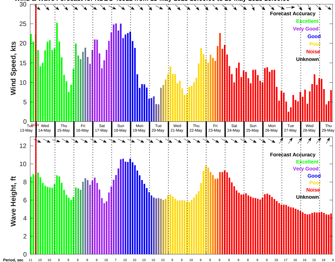
Wind & Wave Forecast for NDBC 46011 from 13-May-2025 16:00:00 to 29-May-2025 16:00:00
