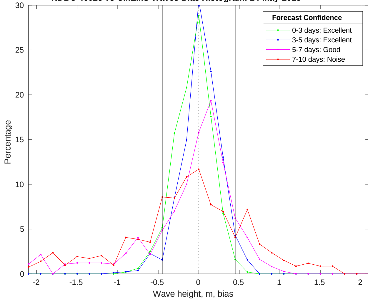
NDBC 46028 vs CMEMS Waves Bias Histogram: 14-May-2025
