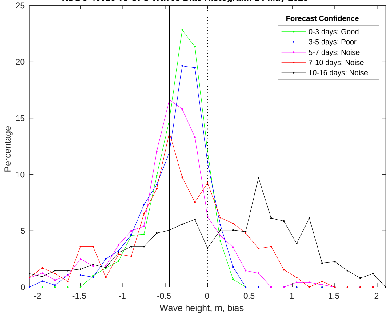
NDBC 46028 vs GFS Waves Bias Histogram: 14-May-2025
