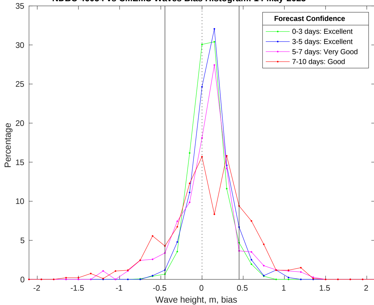
NDBC 46054 vs CMEMS Waves Bias Histogram: 14-May-2025
