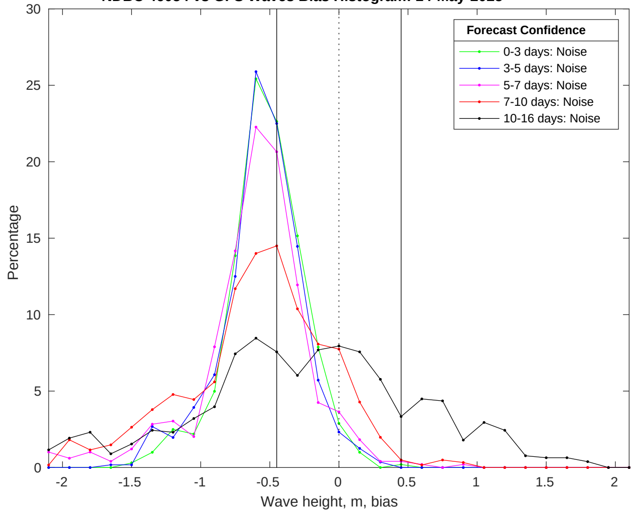
NDBC 46054 vs GFS Waves Bias Histogram: 14-May-2025
