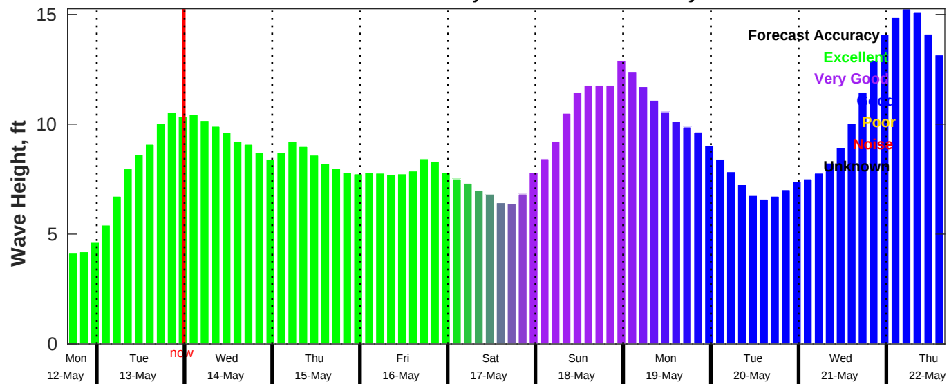
CMEMS Wave Forecast for NDBC 46054 from 12-May-2025 16:00:00 to 22-May-2025 16:00:00
