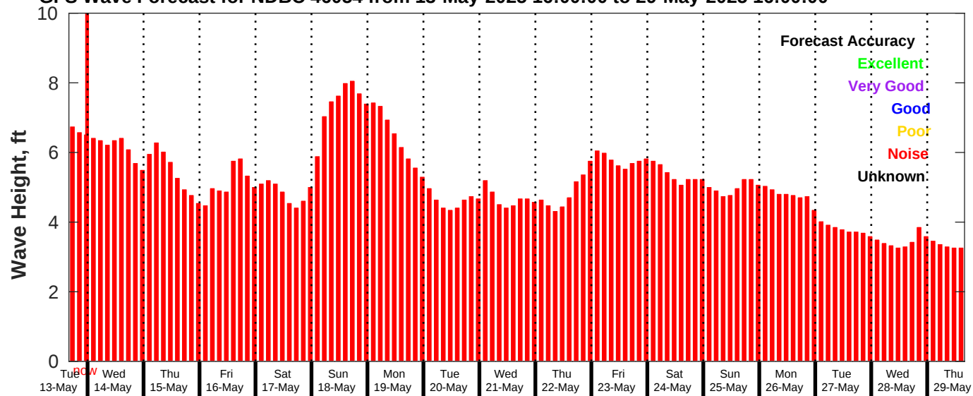
GFS Wave Forecast for NDBC 46054 from 13-May-2025 16:00:00 to 29-May-2025 16:00:00
