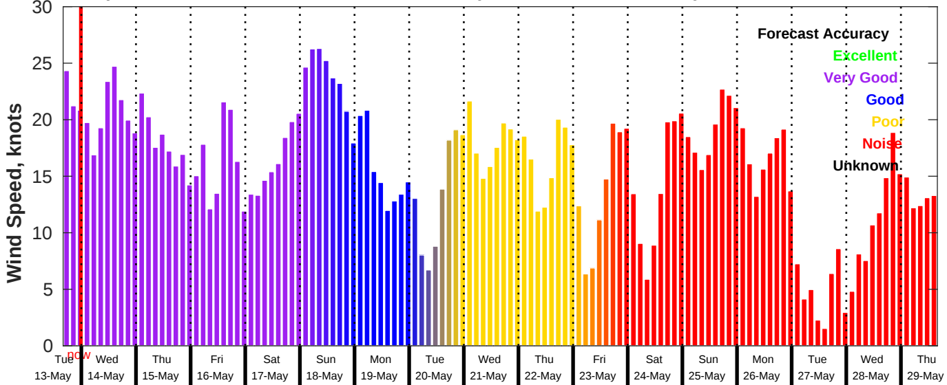
GFS Wind Speed Forecast for NDBC 46054 from 13-May-2025 16:00:00 to 29-May-2025 16:00:00
