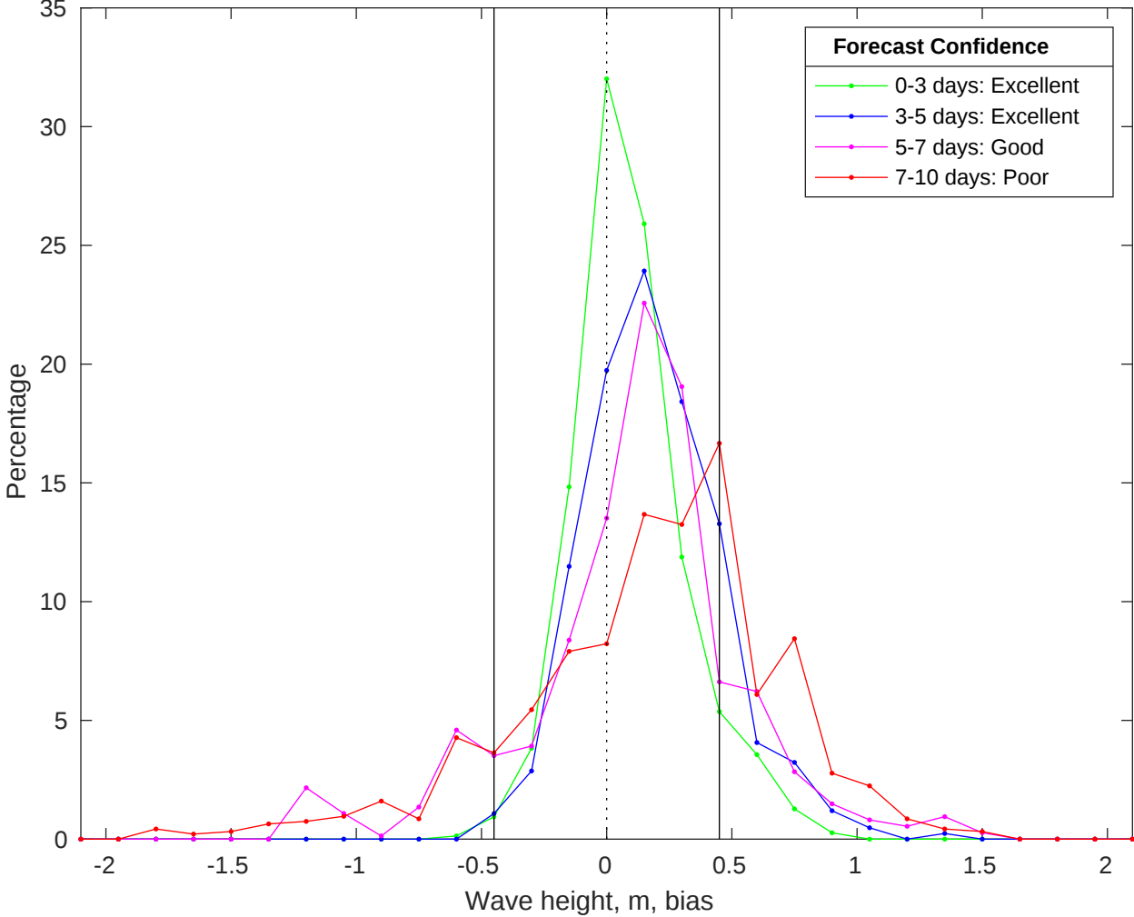
NDBC 46069 vs CMEMS Waves Bias Histogram: 14-May-2025
