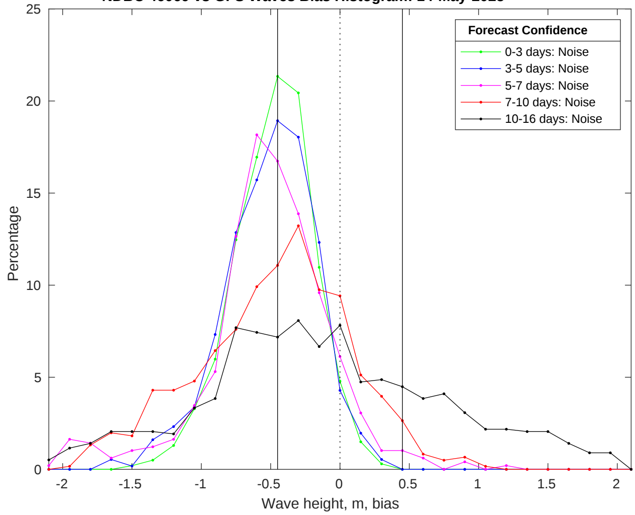
NDBC 46069 vs GFS Waves Bias Histogram: 14-May-2025
