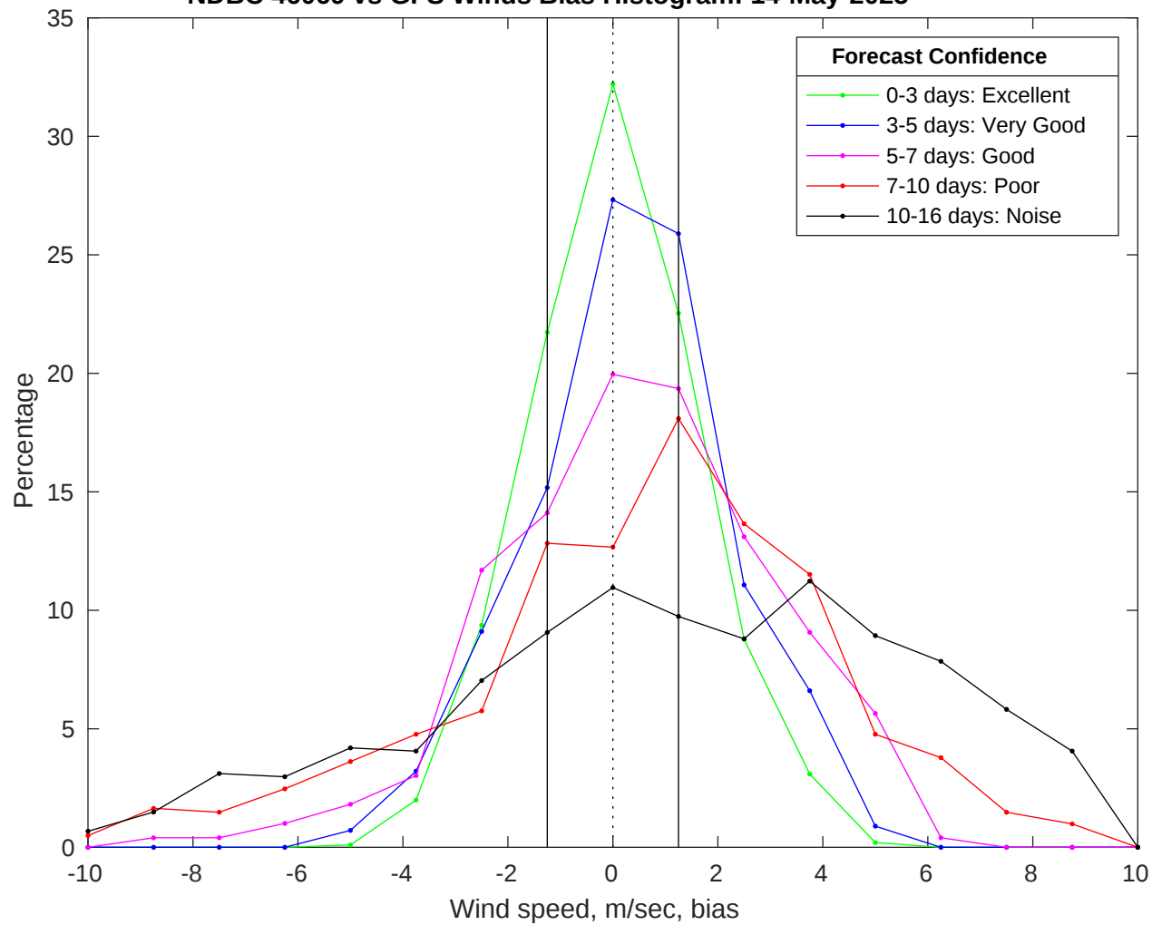
NDBC 46069 vs GFS Winds Bias Histogram: 14-May-2025
