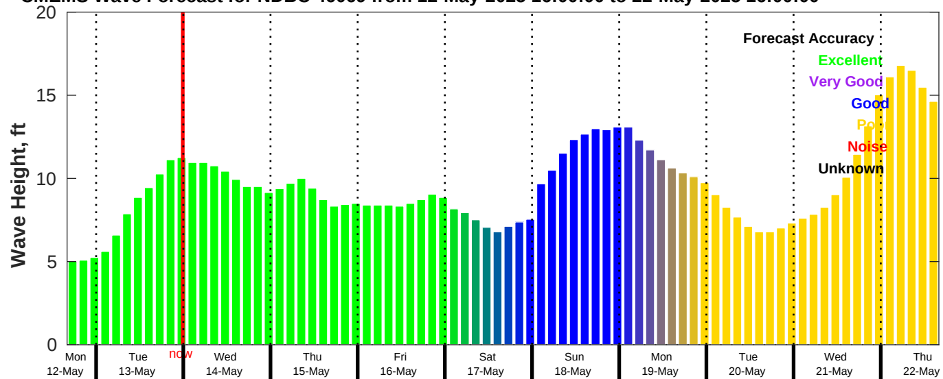
CMEMS Wave Forecast for NDBC 46069 from 12-May-2025 16:00:00 to 22-May-2025 16:00:00
