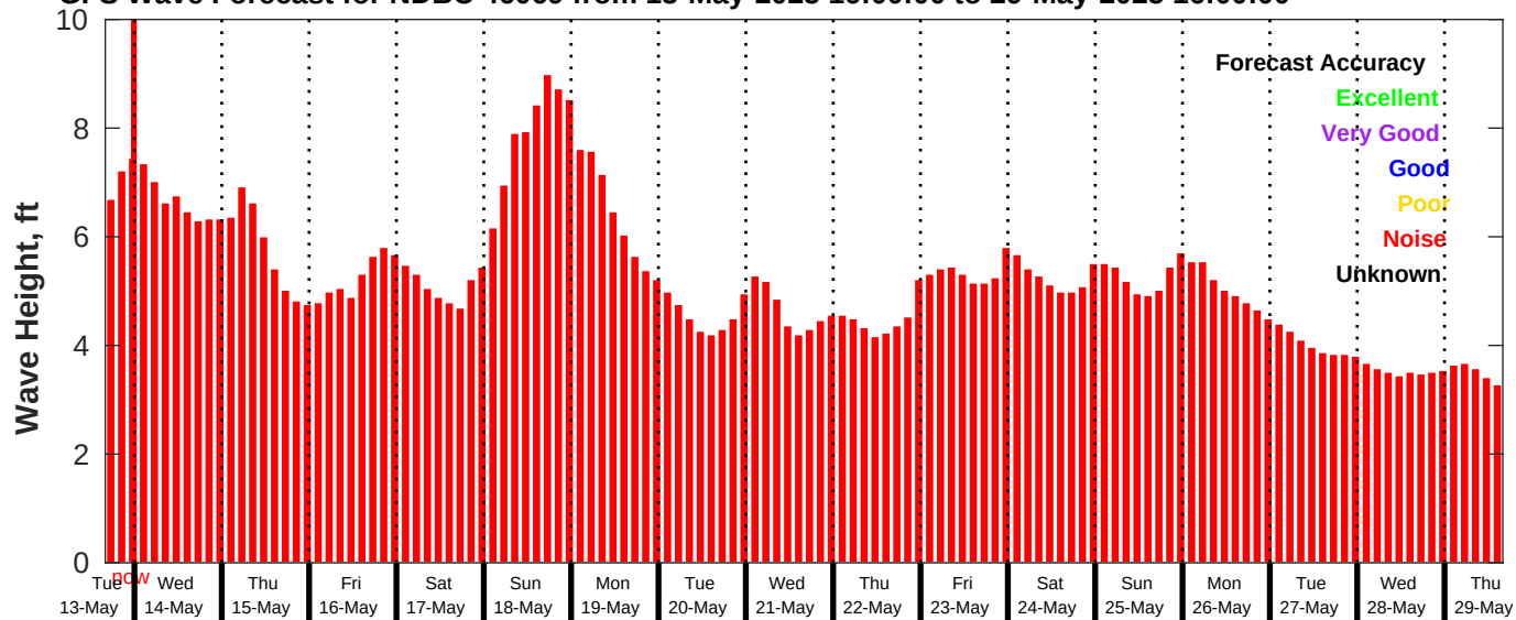
GFS Wave Forecast for NDBC 46069 from 13-May-2025 16:00:00 to 29-May-2025 16:00:00
