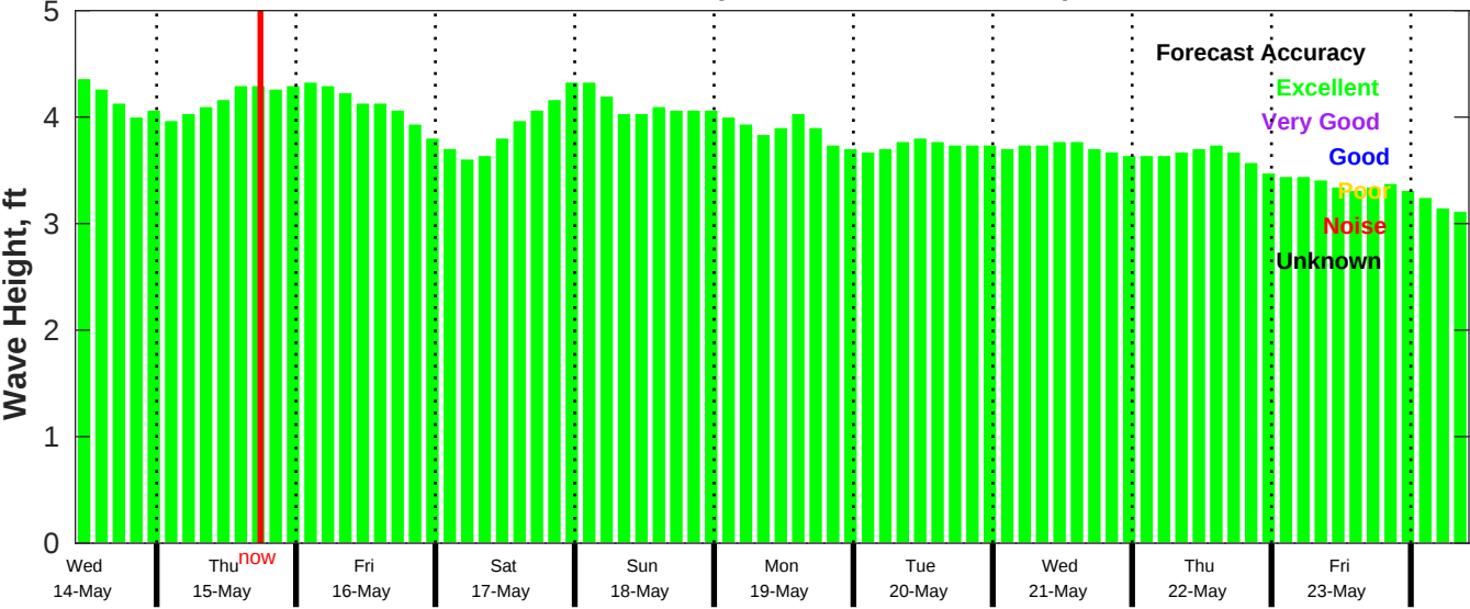
CMEMS Wave Forecast for NDBC 52211 from 13-May-2025 10:00:00 to 23-May-2025 10:00:00
