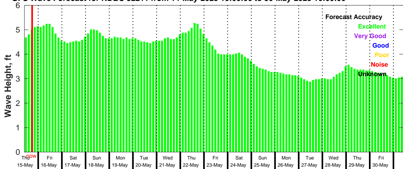
GFS Wave Forecast for NDBC 52211 from 14-May-2025 10:00:00 to 30-May-2025 10:00:00
