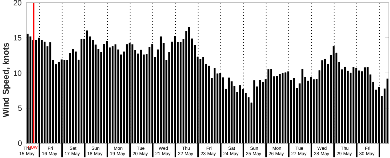
GFS Wind Speed Forecast for NDBC 52211 from 14-May-2025 10:00:00 to 30-May-2025 10:00:00
