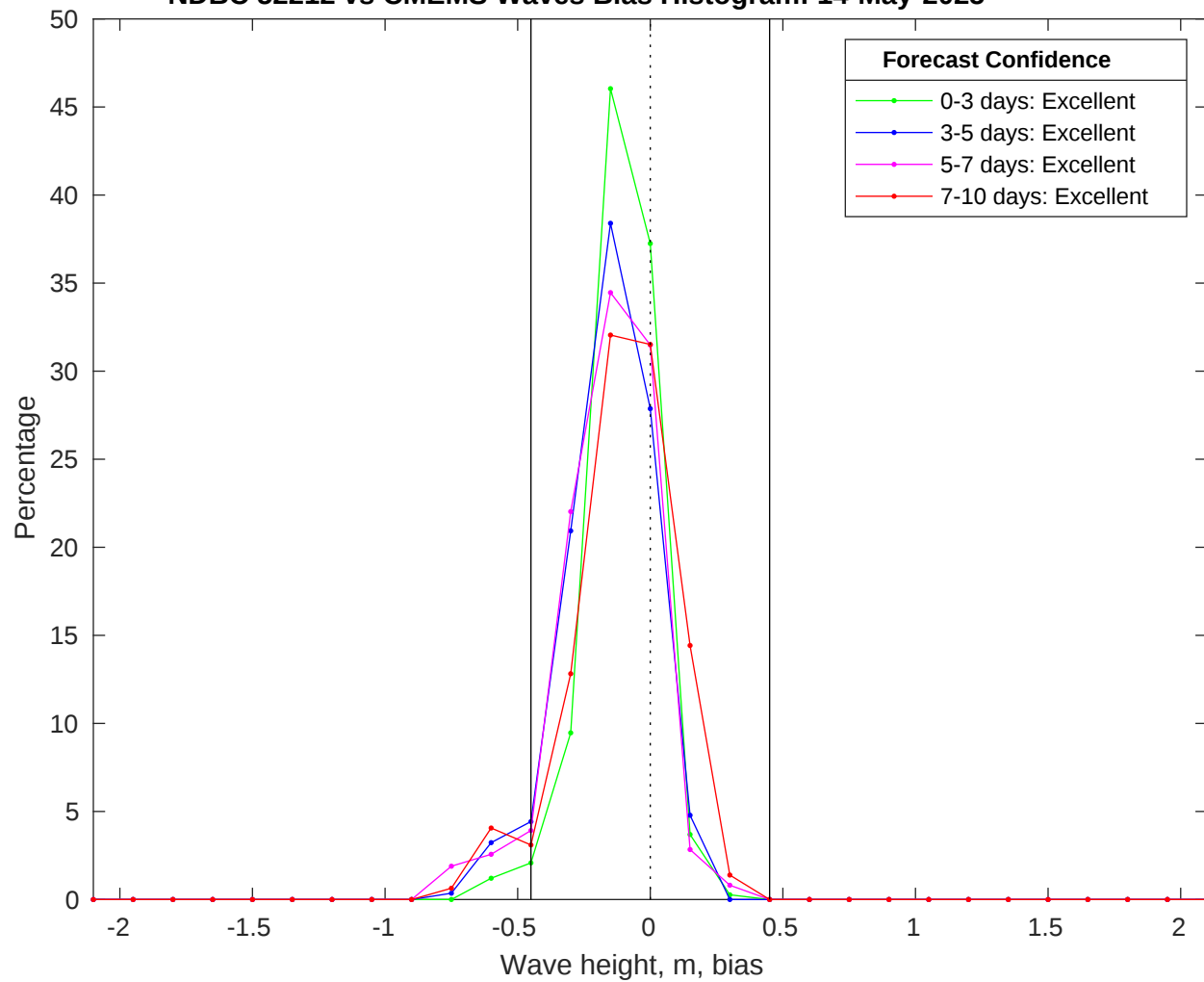
NDBC 52212 vs CMEMS Waves Bias Histogram: 14-May-2025
