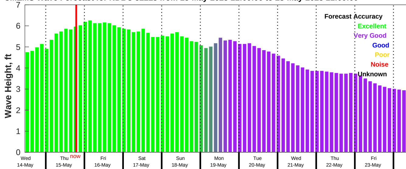
CEEMS Wave Forecast for NDBC 52213 from 13-May-2025 11:00:00 to 23-May-2025 11:00:00
