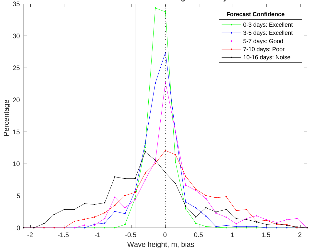
NDBC 41004 vs GFS Waves Bias Histogram: 15-May-2025
