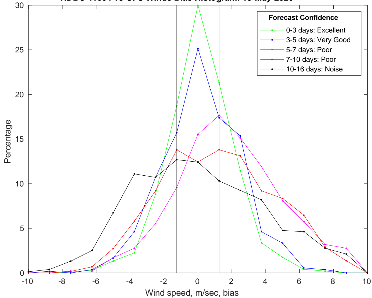
NDBC 41004 vs GFS Winds Bias Histogram: 15-May-2025
