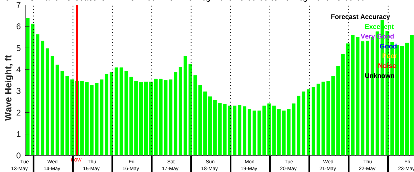
CMEMS Wave Forecast for NDBC 41004 from 13-May-2025 19:00:00 to 23-May-2025 19:00:00
