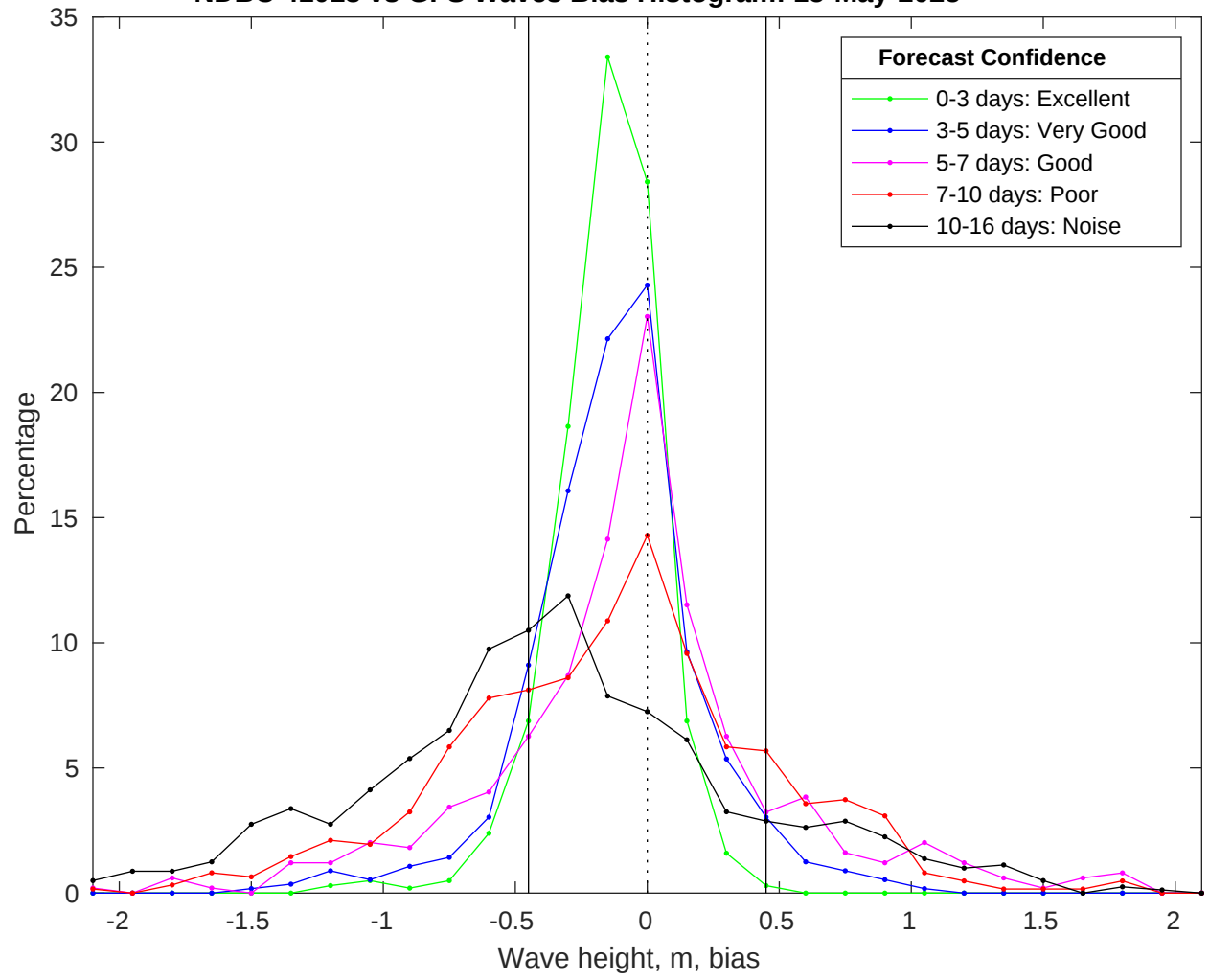
NDBC 41013 vs GFS Waves Bias Histogram: 15-May-2025
